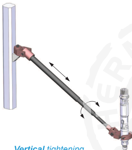
Vertical tightening
